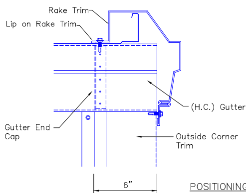
POSITIONING STANDARD GUTTER
