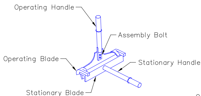
MANUAL SEAMING TOOL
