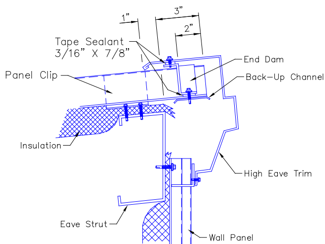
PANEL ENDS AT HIGH EAVE
