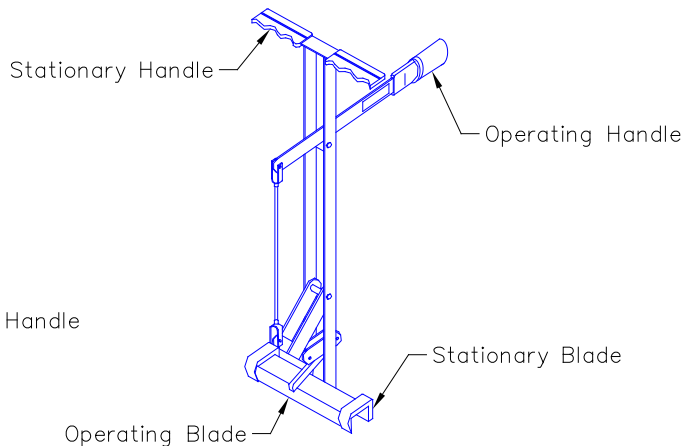
STAND-UP SEAMING TOOL
