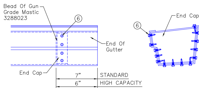
END CAP LOCATION
