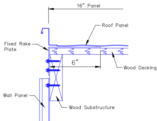
0" START DIMENSION
