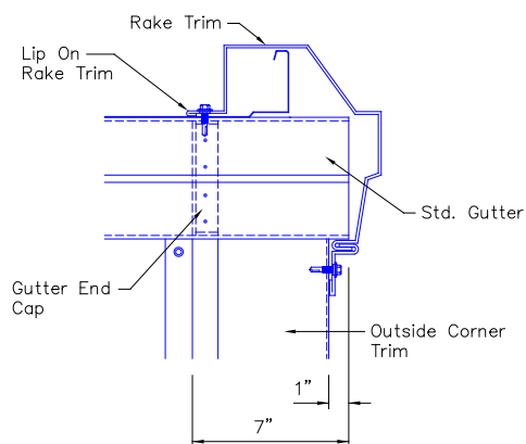
POSITIONING STANDARD GUTTER
