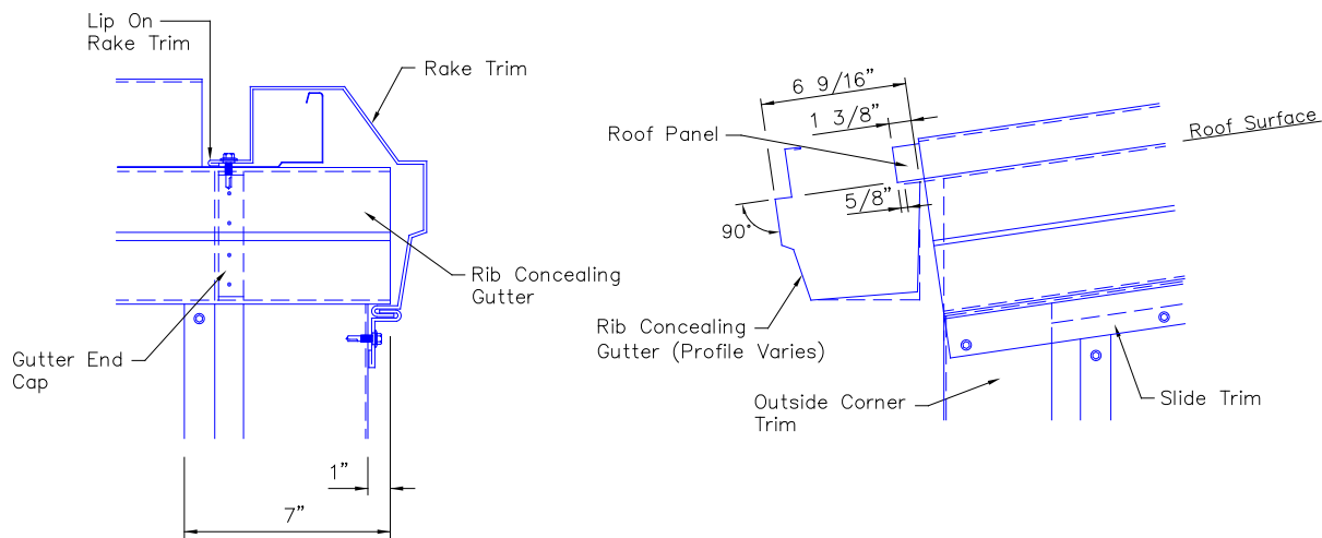
POSITIONING RIB CONCEALING GUTTER
