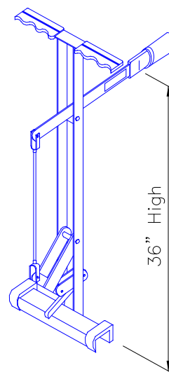
STAND-UP SEAMER 255139
