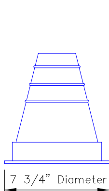
2368-004 PIPE FLASHING FOR PIPES WITH O.D. OF 1/4" TO 4"
