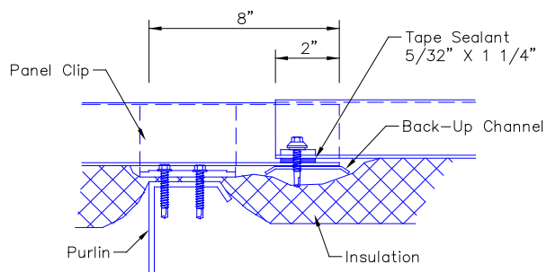
PANEL END LAP AT PURLIN
