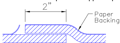
OVERLAP MASTIC
