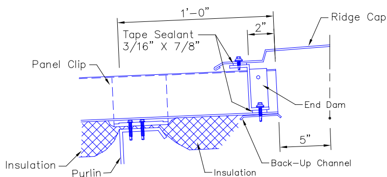
PANEL ENDS AT RIDGE
