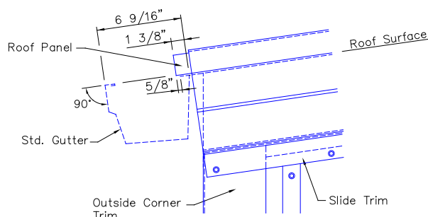
POSITIONING STANDARD GUTTER
