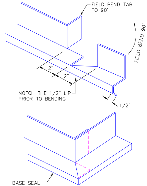
ILLUS. 5.13 BASE SEAL AT BOTTOM OF WALL PANEL
