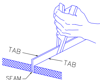
ILLUS. 5.2 STEP NO. 1
