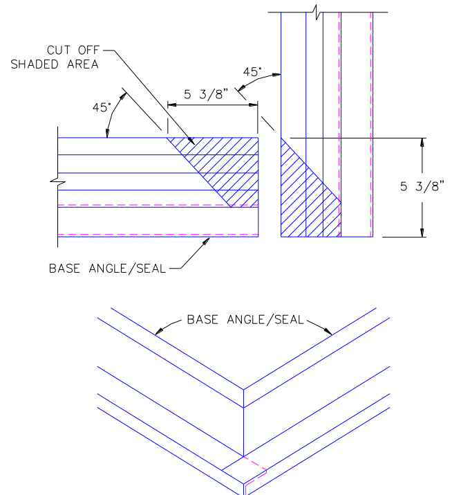
ILLUS. 5.14 BASE ANGLE/SEAL AT BOTTOM OF WALL PANEL
