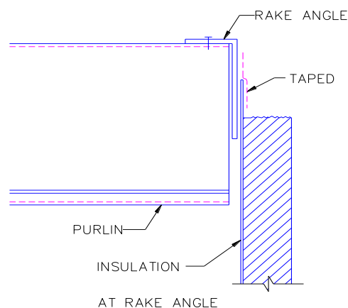
ILLUS. 5.7 INSULATION TAPED AT TOP
