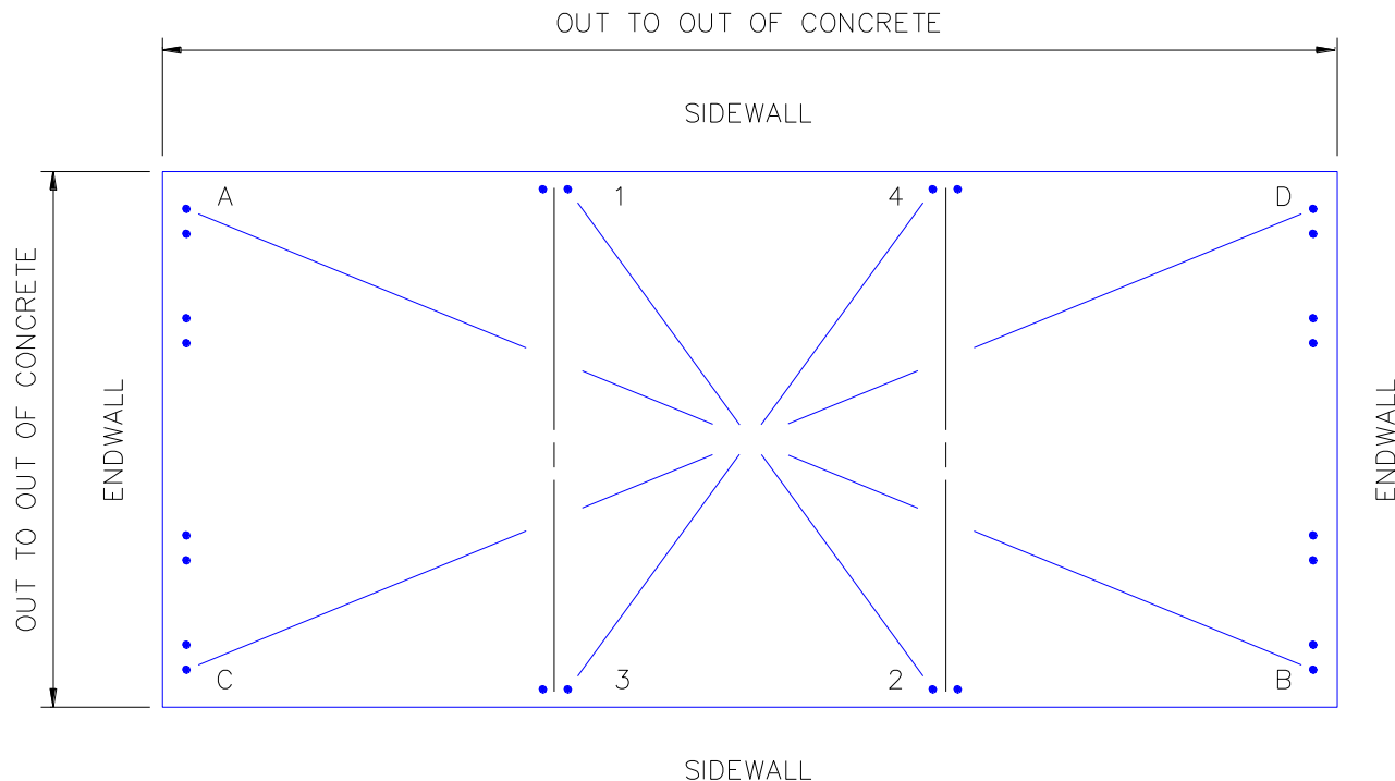
ILLUS. 2.1 CHECKING FOUNDATION
