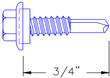
ILLUS. 4.1 STITCH SCREW
