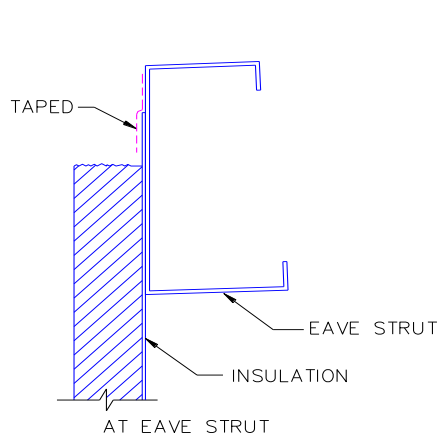
ILLUS. 5.7 INSULATION TAPED AT TOP
