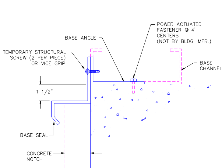
ILLUS. 5.13 BASE SEAL AT BOTTOM OF WALL PANEL
