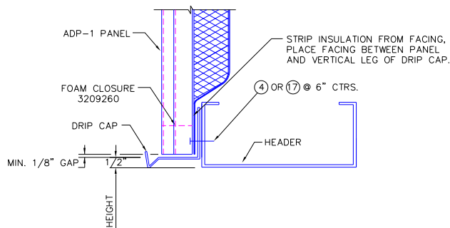
ILLUS. 6.6 PANELS AT HEADER
