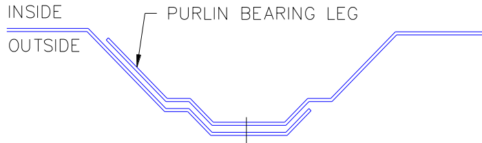
ILLUS. 5.17 PANEL SIDELAP
