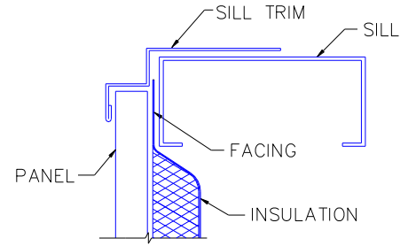
ILLUS. 5.11 AT SILL
