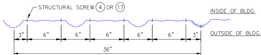
ILLUS. 4.5 STRUCTURAL SCREW PATTERNS FOR ADP-1 PANELS
