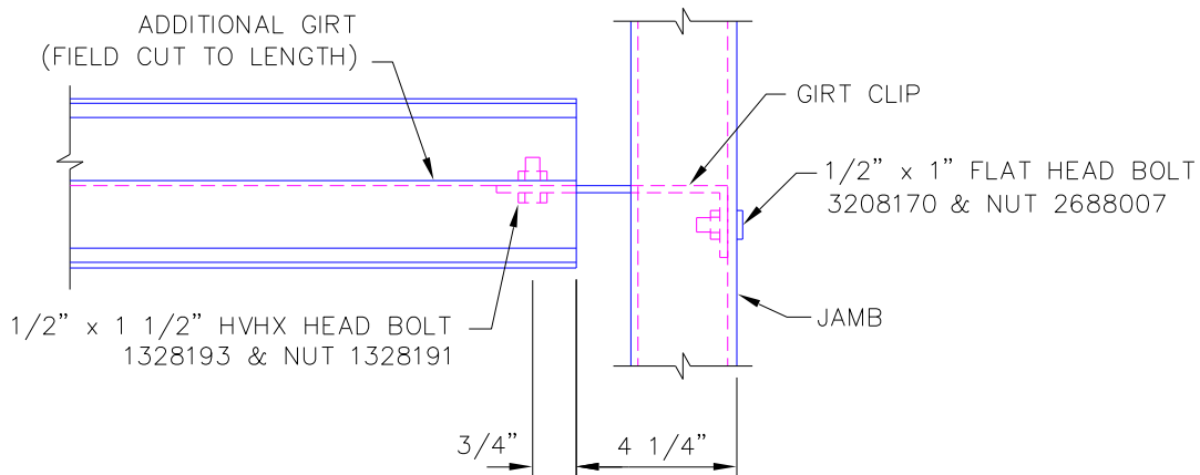
ILLUS. 6.27 ATTACHING ADDITIONAL GIRTS TO JAMB
