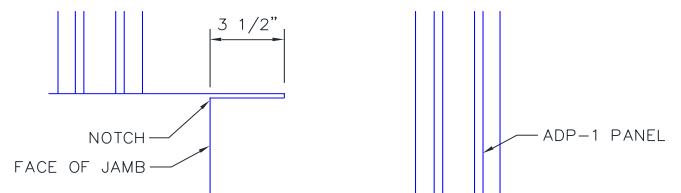
ILLUS. 6.3 NOTCH PANELS FOR DRIP CAP
