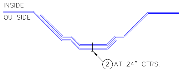
ILLUS. 5.24 ADP-1 PANEL SIDELAP
