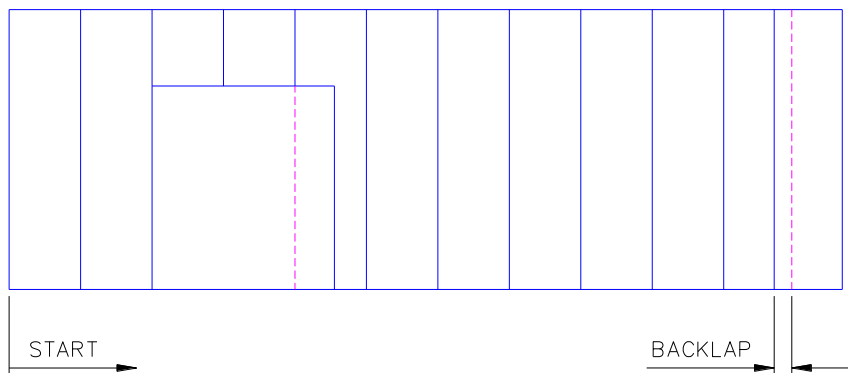
ILLUS. 5.18 FRONT SIDEWALL ELEVATION (VIEWED FROM OUTSIDE OF BUILDING)
