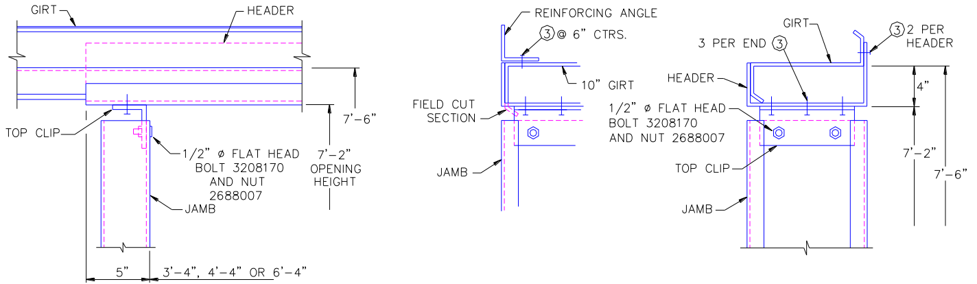
ILLUS. 6.17 HEADER AND JAMB CONNECTION TO GIRTS
