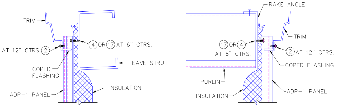
ILLUS. 5.29 ROOF PERIMETER TRIMS AT TOP OF WALL PANEL
