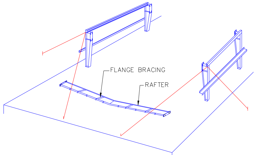
ILLUS. 2.3 ASSEMBLING RAFTER
