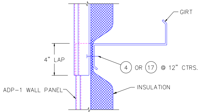
ILLUS. 5.23 WALL PANEL ENDLAP
