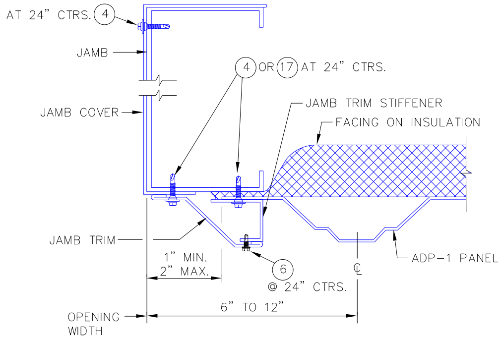
ILLUS. 6.4 TRIMS AT SIDES OF FRAMED OPENING
