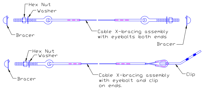
ILLUS. 2.5 CABLE ASSEMBLIES
