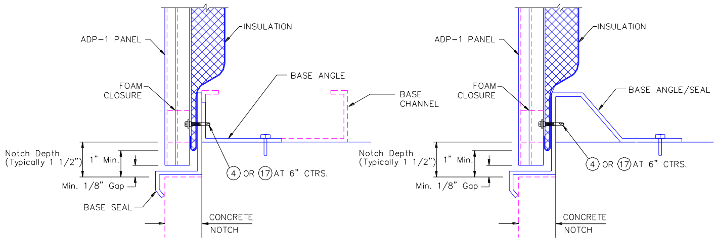
ILLUS. 5.15 FOAM CLOSURES AT BASE OF WALL
