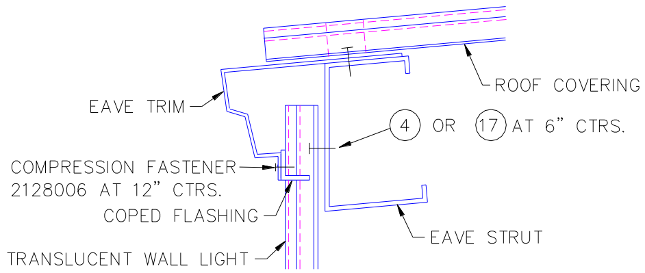
ILLUS. 6.37 ATTACHING TRIM TO TRANSLUCENT WALL LIGHT
