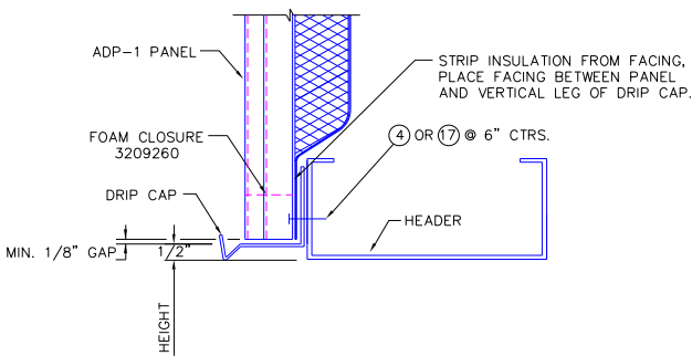
ILLUS. 6.6 PANELS AT HEADER
