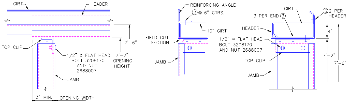
ILLUS. 6.26 HEADER AND JAMB CONNECTIONS TO GIRTS
