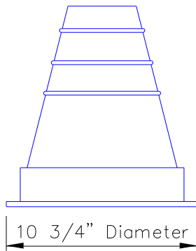
2368-005 PIPE FLASHING FOR PIPES WITH O.D. OF 4" TO 7"
