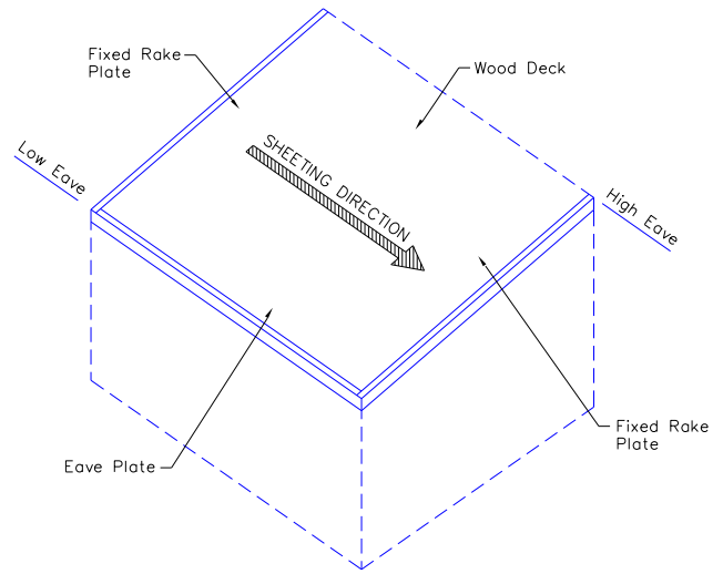
SINGLE SLOPE BLDG.
