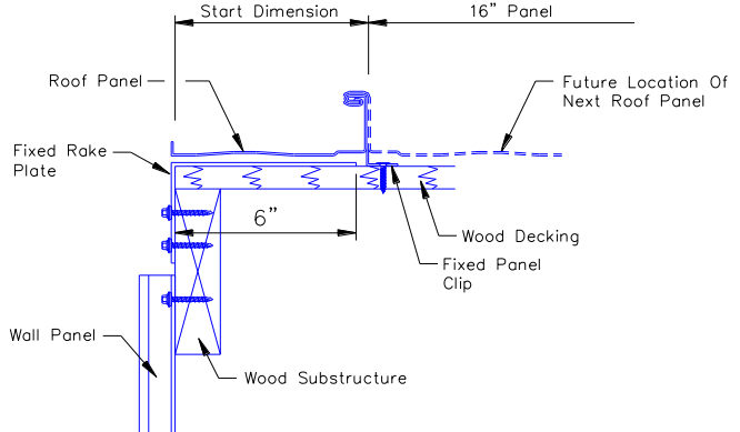
START DIMENSION GREATER THAN 0"
