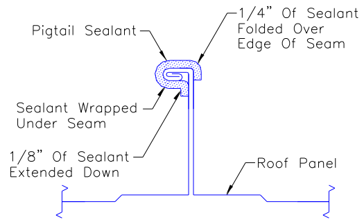
PIGTAIL SEALANT AT RIDGE OR HIGH EAVE
