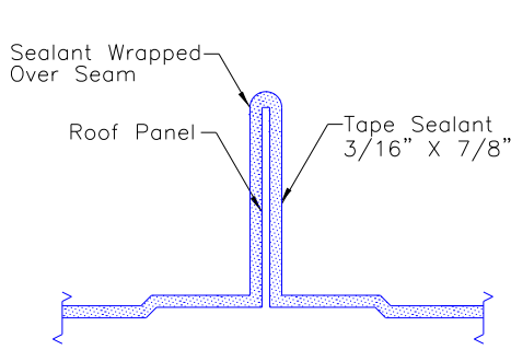
3/16" X 7/8" TAPE SEALANT AT RIDGE OR HIGH EAVE
