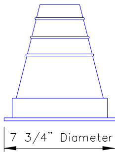
2368-004 PIPE FLASHING FOR PIPES WITH O.D. OF 1/4" TO 4"
