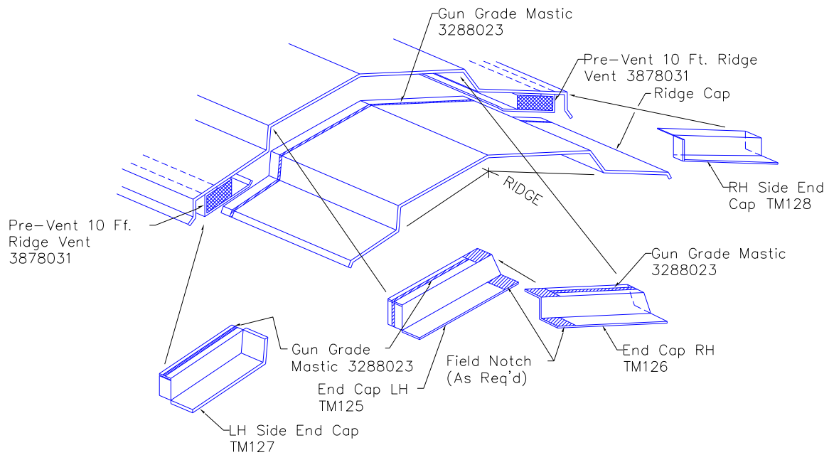
PARTIAL ASSEMBLED
