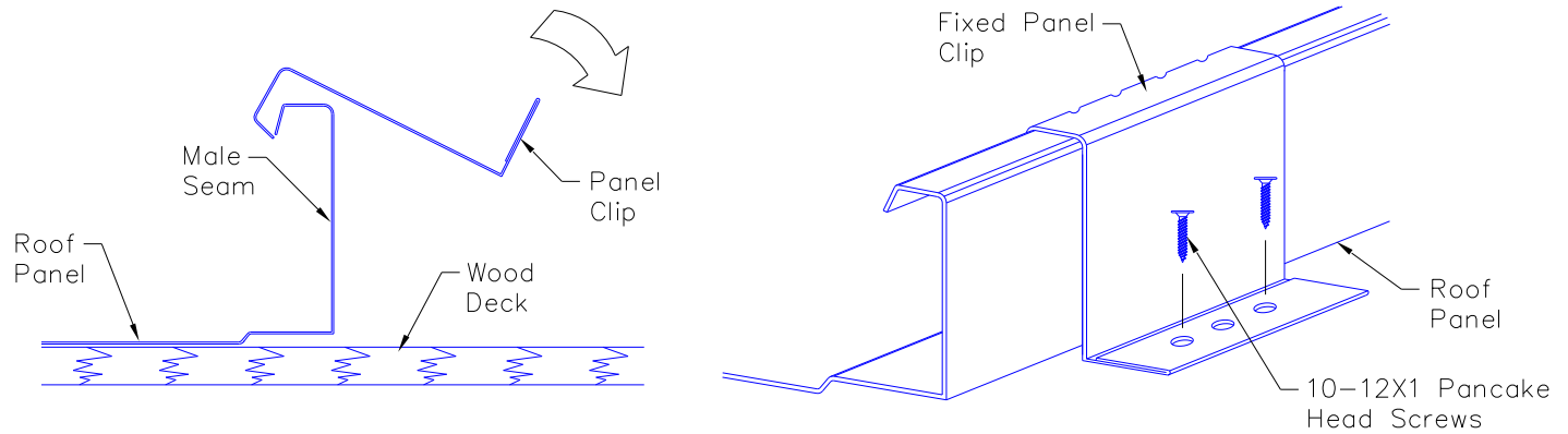
CLIP AND PANEL ASSEMBLY
