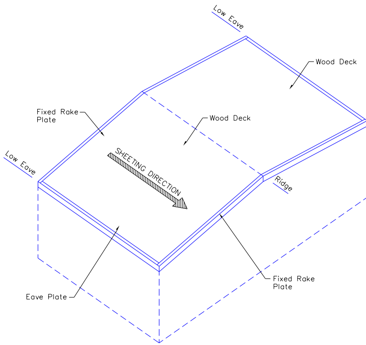
GABLED BLDG.
