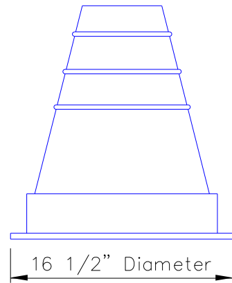
2368-006 PIPE FLASHING FOR PIPES WITH O.D. OF 7" TO 13"
