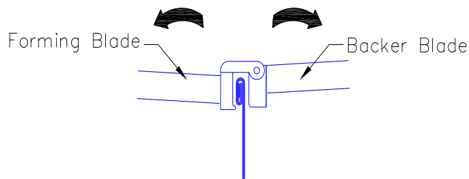
FLATTENING SEAM
