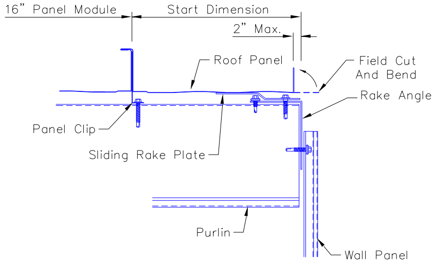
START DIMENSION GREATER THAN 0"
