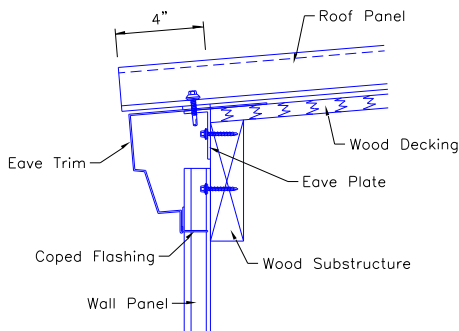
PANEL OVERHANG WITH EAVE TRIM
