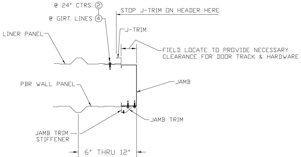
AT JAMB WITH PBR WALL PANEL
