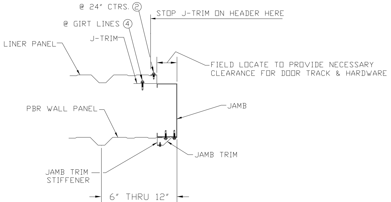
AT JAMB WITH PBR WALL PANEL
