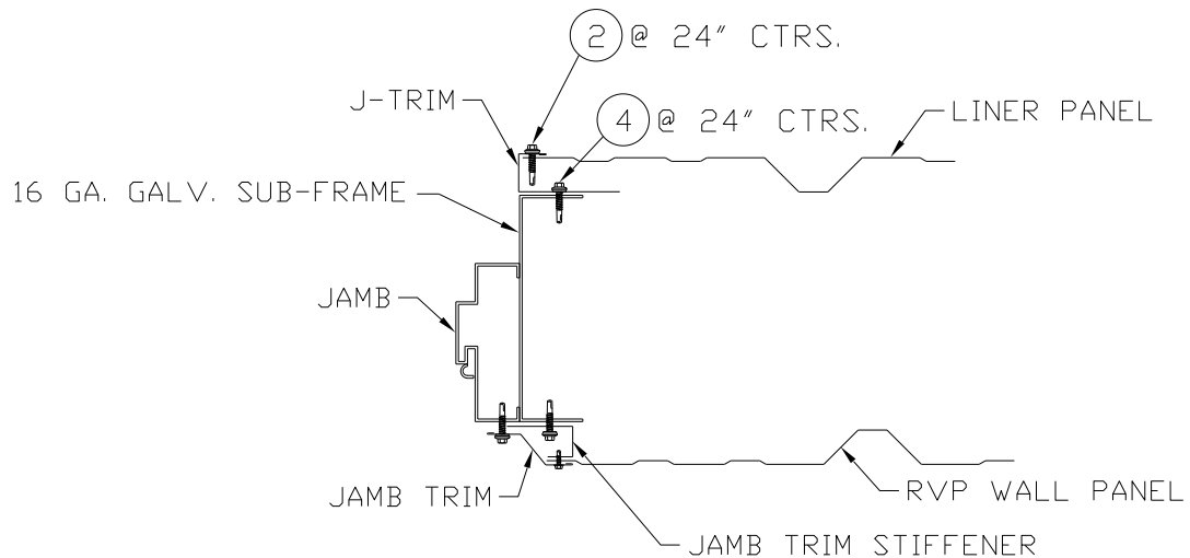
AT JAMB WITH RVP PANEL
