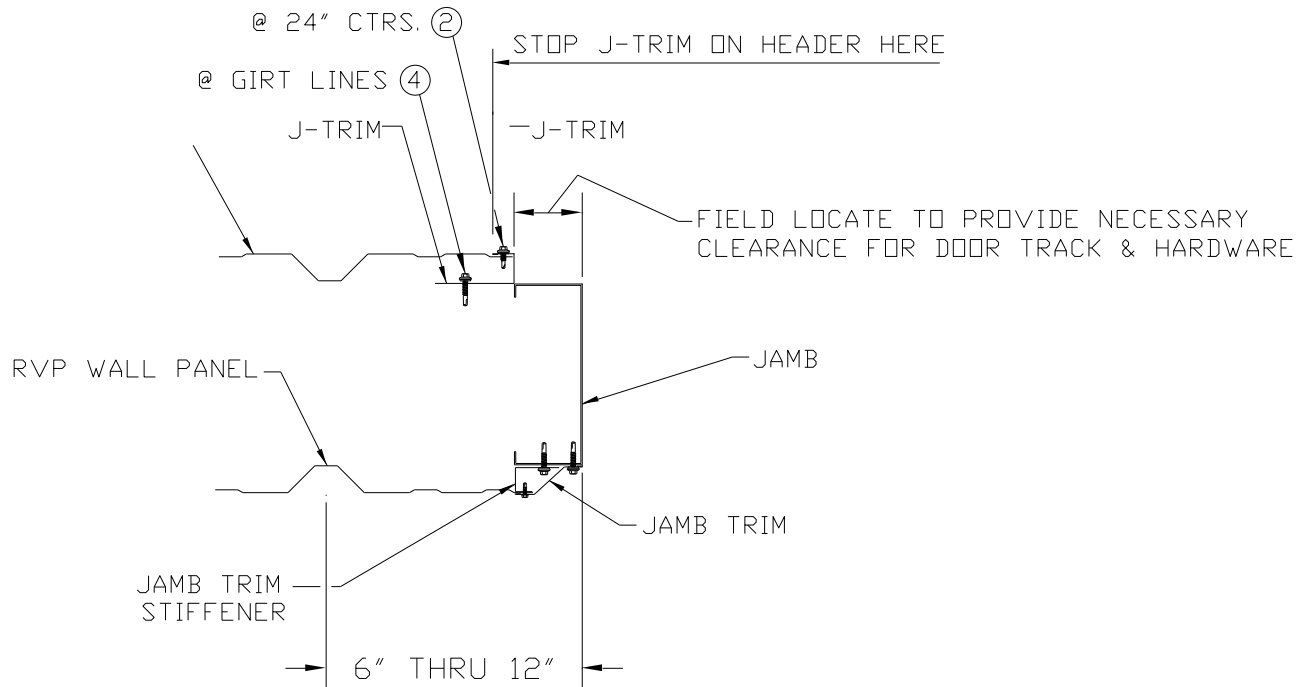
AT JAMB WITH RVP WALL PANEL
