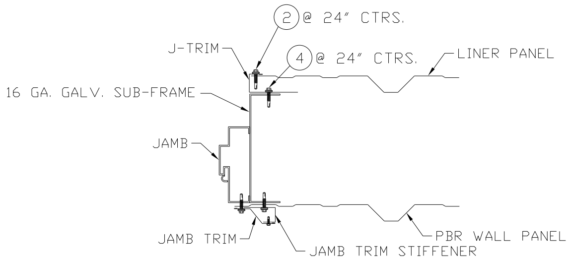
AT JAMB WITH PBR PANEL
